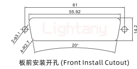
板前安装开孔 (Front Install Cutout)
