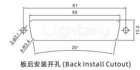
板后安装开孔 (Back Install Cutout)
